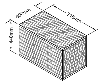
RAINSMART ELLIPSE SINGLE TANK MODULE
