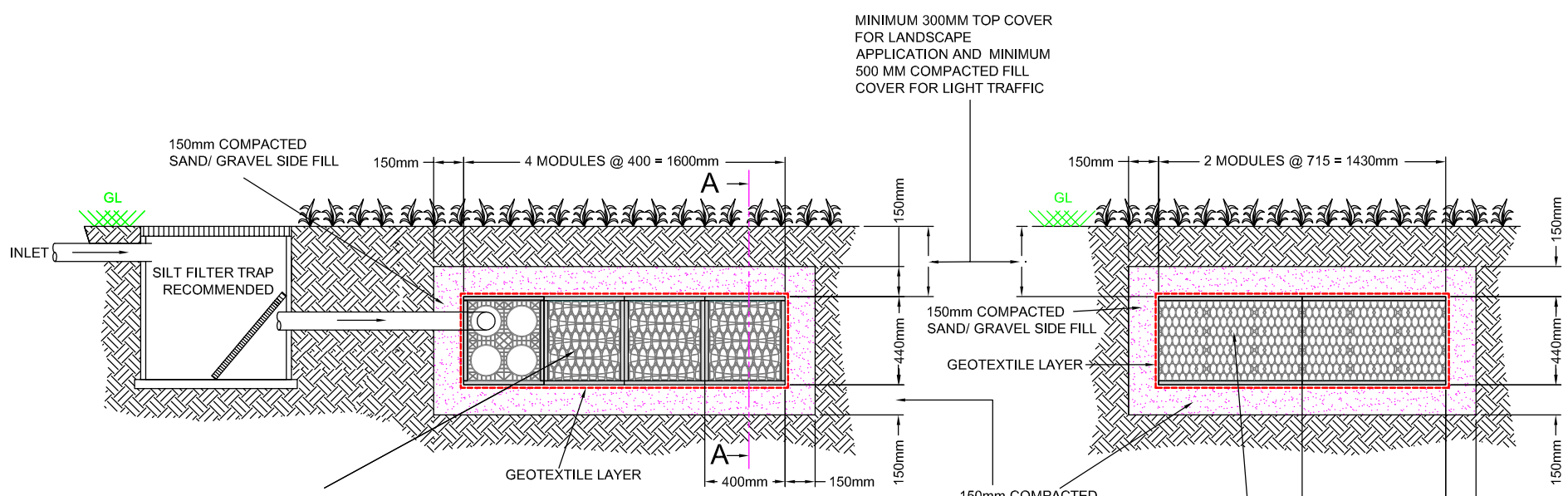
FRONT VIEW
